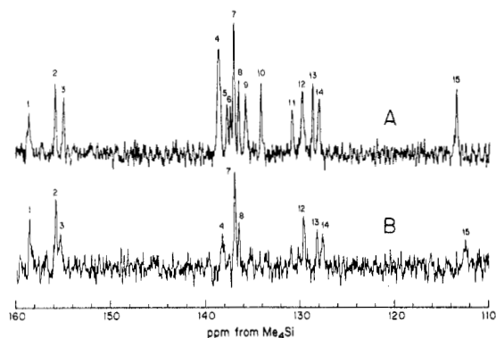
Figure 7. Region of aromatic carbons (and C^\gamma of arginines) in convolution-difference natural-abundance ^{13}C NMR spectra of P. aeruginosa azurin (in H_2O , 0.05 M ammonium acetate, 31 ^\circ C ). Each spectrum was recorded at 14.2 kG, with a 20-mm probe, noise-modulated off-resonance proton decoupling, and a recycle time of 1.1 s. (A) Cu(I) azurin (7.4 mM), pH 5.2, 65 536 scans. (B) Cu(II) azurin (5.8 mM), pH 5.3, 131 072 scans. Taken from ref 10.
